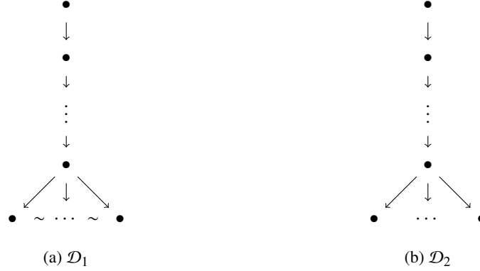
Figure 1: Types of top-truncated preferences in two domains: \mathcal{D}_1 and \mathcal{D}_2 .
