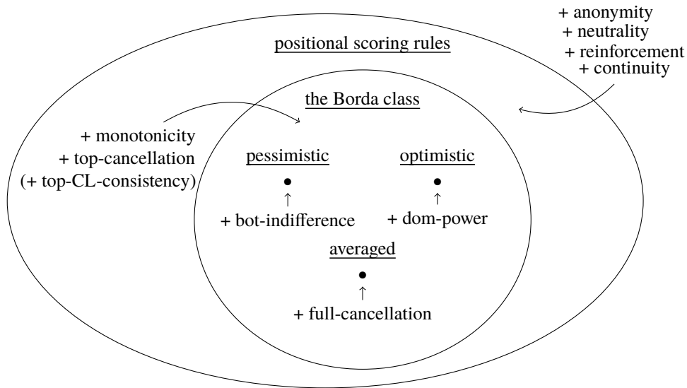
Figure 6: Borda rules for top-truncated preferences and the axioms that characterise them. The axioms next to an arrow indicate those properties that are required in order to obtain a specific class of rules, or a specific rule, within a larger class.
