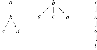
Figure 5: A profile where the pessimistic, the optimistic, and the average Borda rule output different sets of winners: \{b\} , \{a, c\} , and \{a, b\} , respectively.
