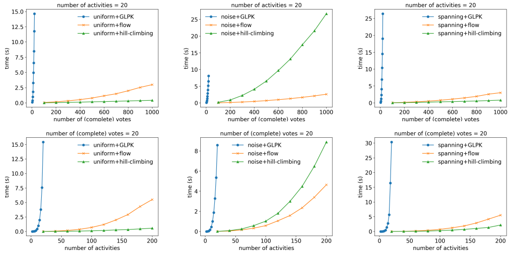
Figure 3: Runtime of the 3 algorithms on inputs from different distributions. The top 3 figures plot the growth of running times when the number of votes grows, and the bottom 3 figures show the running times when the number of activities grows.
