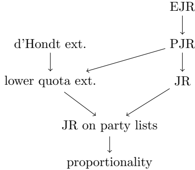
Figure 1: Proportionality axioms and logical implications.
